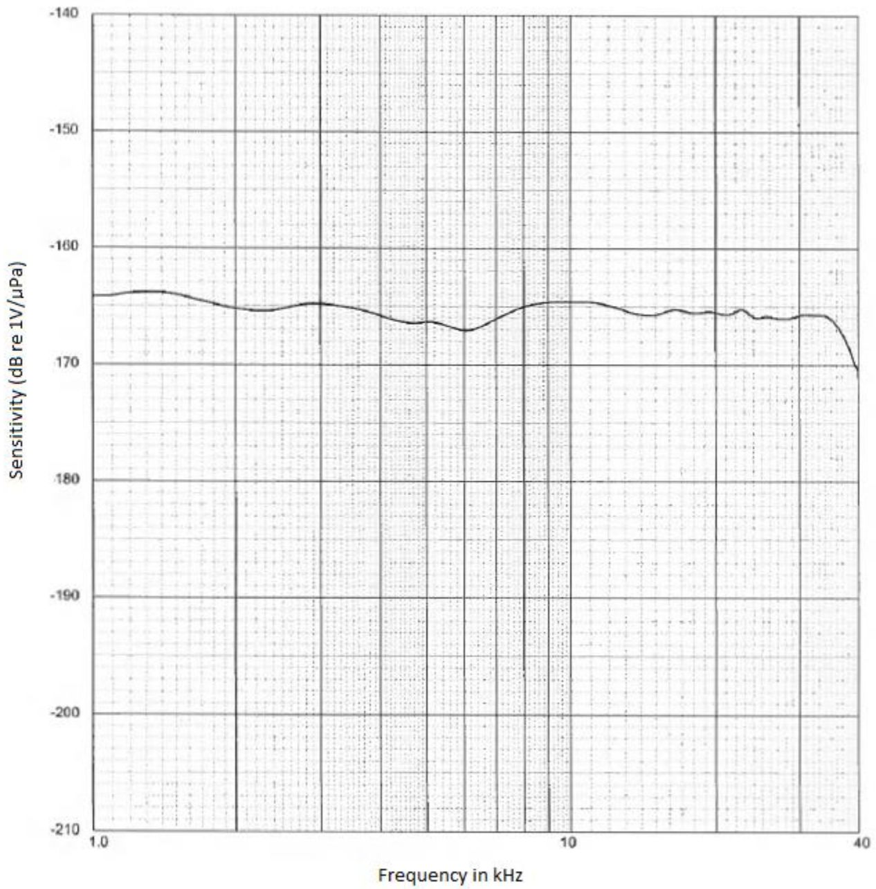
Frequency Response of Hydrophone HTI-96-MIN
